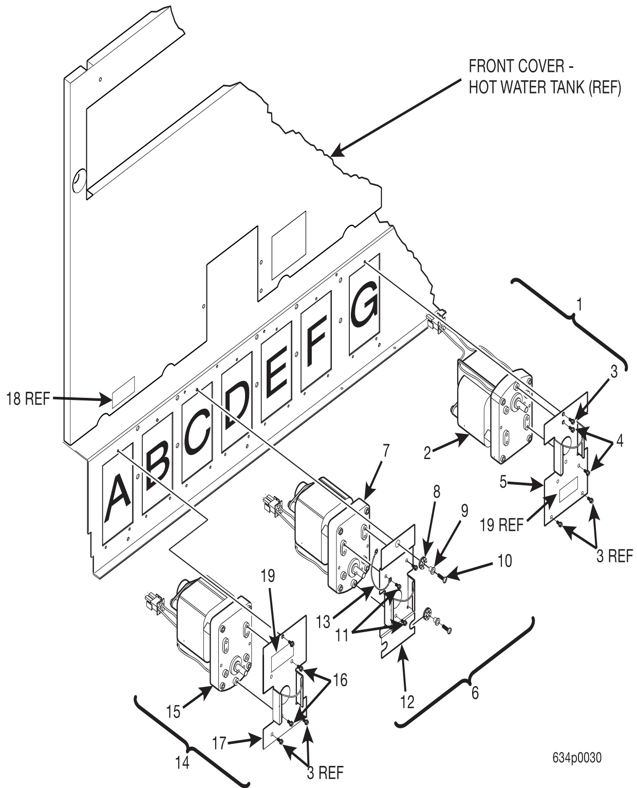
Figure 72. Canister Motor and Plate Assemblies (Continued)
