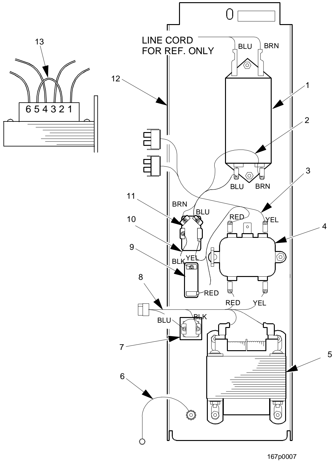
Figure 40. Power Panel Assembly - 230 V - Argentina, Australia, Brazil, Latin America (220 V), New Zealand, Singapore, U.K.
